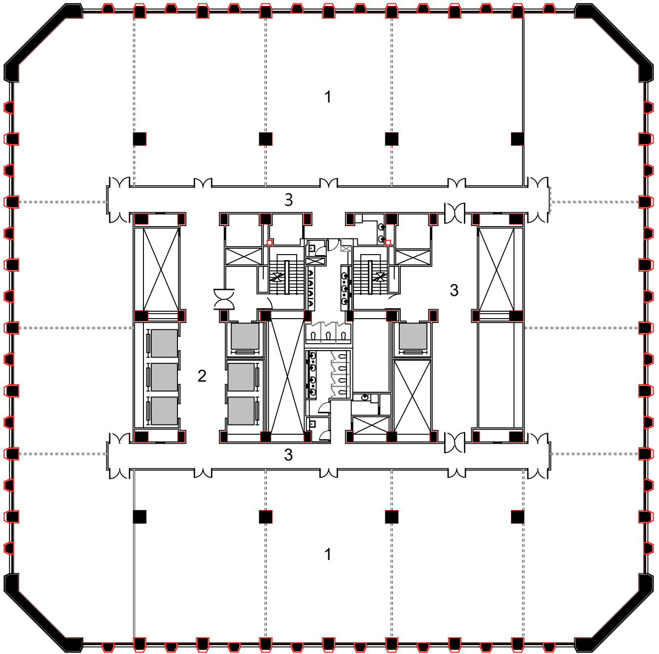
Typical floor plan (3~13)
