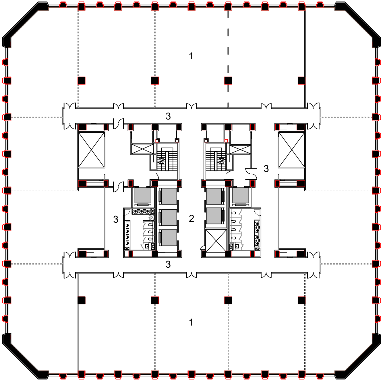
Typical floor plan (24~33)
